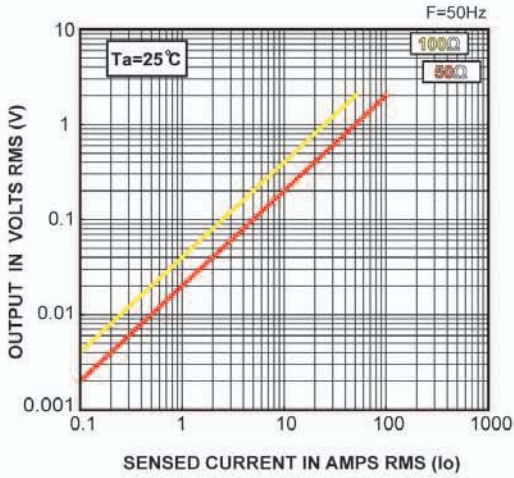
JH3V
