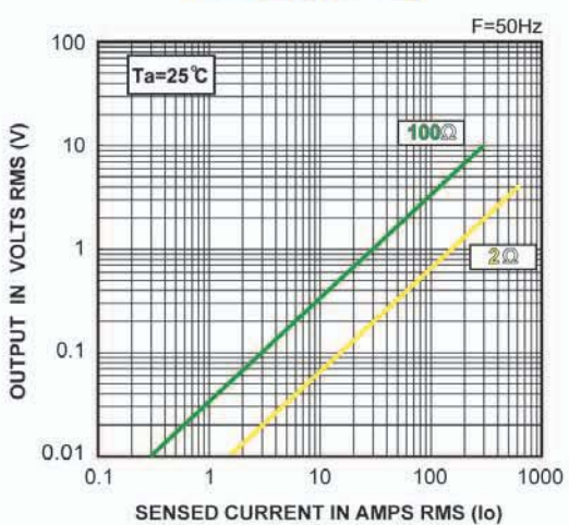
CT3000
