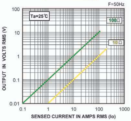
CT1000
