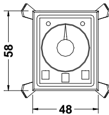
NH3-C + Y-40 Adapter
