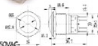
S2201A 22mm不銹鋼金屬平面環形燈無段開關
