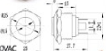
S22102A 22mm不銹鋼金屬弧形無段開關
