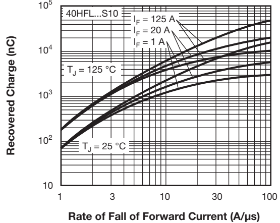
Fig. 24 - Typical Recovered Charge vs. Rate of Fall of Forward Current, 40HFL...Series
