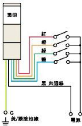
閃光蜂鳴型(MS)
