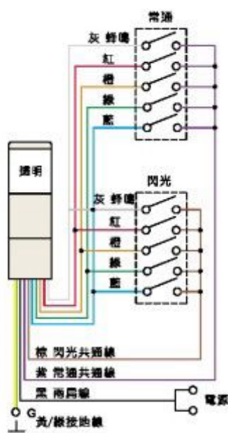
閃光蜂鳴型(MS)
