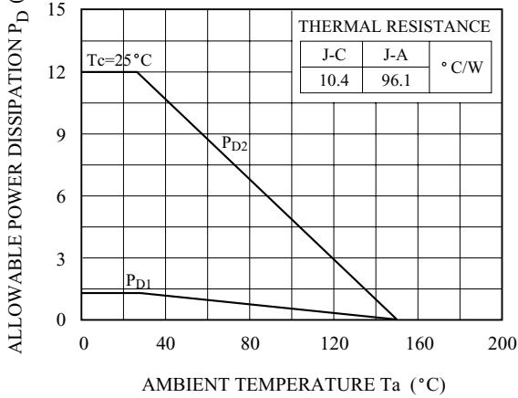
Fig. 10 P_D - T_a (AF-Type : DPAK)
